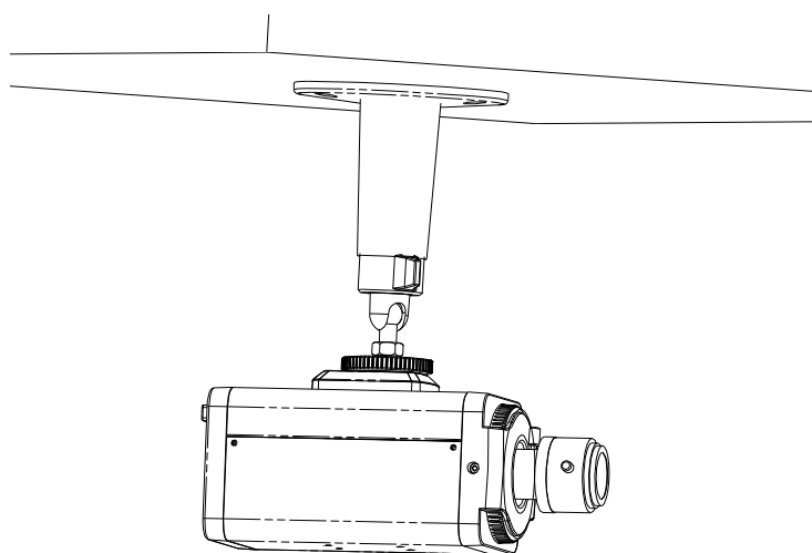
Fig 2.2.3 Fix Lens
