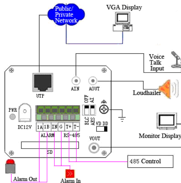
Fig 2.2.8 Topological Graph of Network Camera
