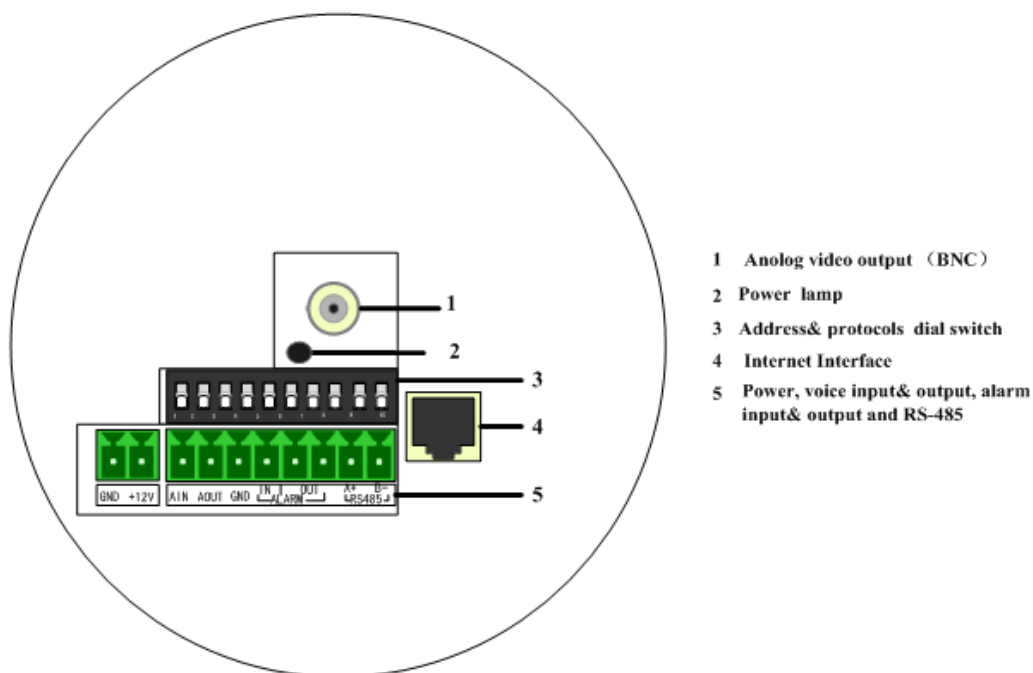
Fig. 2.1.7 Rear Panel of DS-2CD702, DS-2CD712, DS-2CD732, DS-2CD792 series
