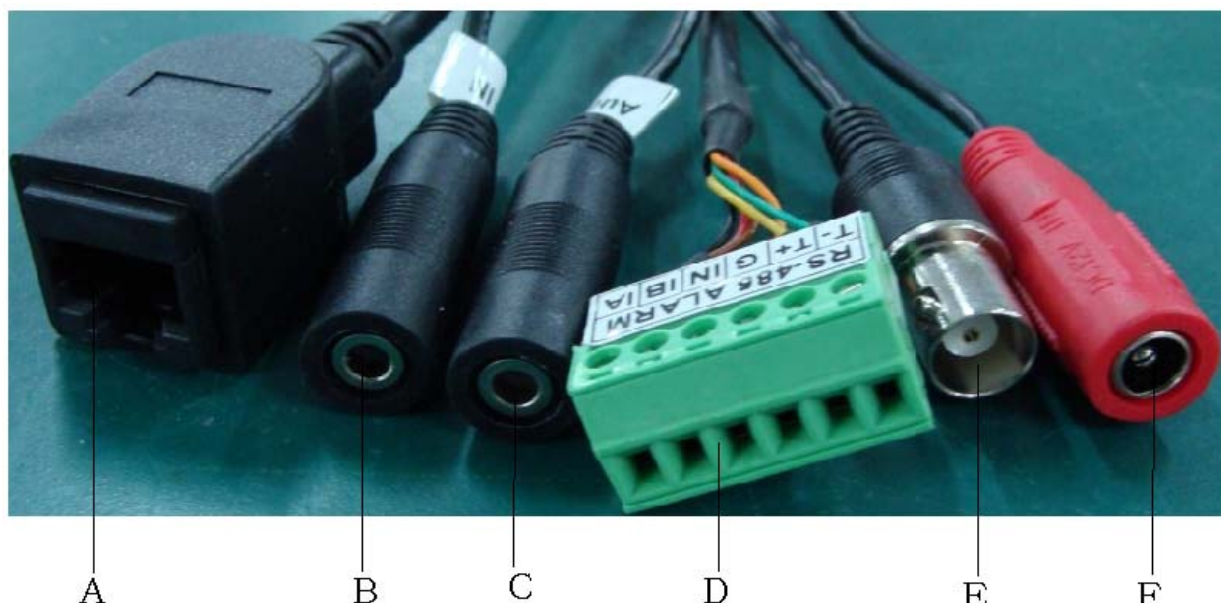
Fig 2.1.8 Rear Panel of DS-2CD802/812/892P-IR1/3/5 series camera
