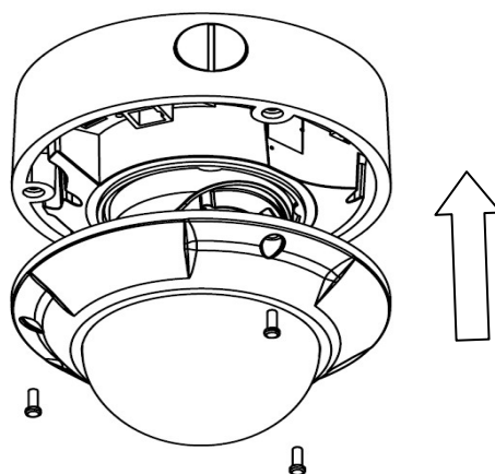
Fig. 2.2.10 Install the Cover
