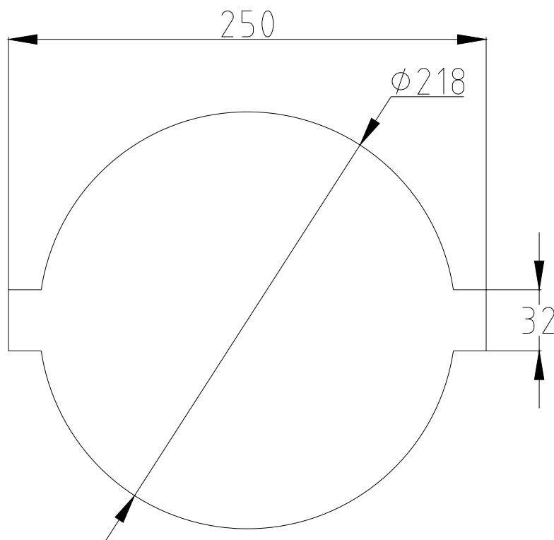
Drill Drawing
