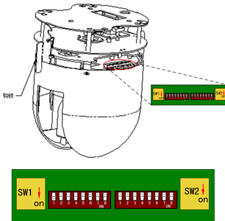
1: SW1 Address DIP Switch
