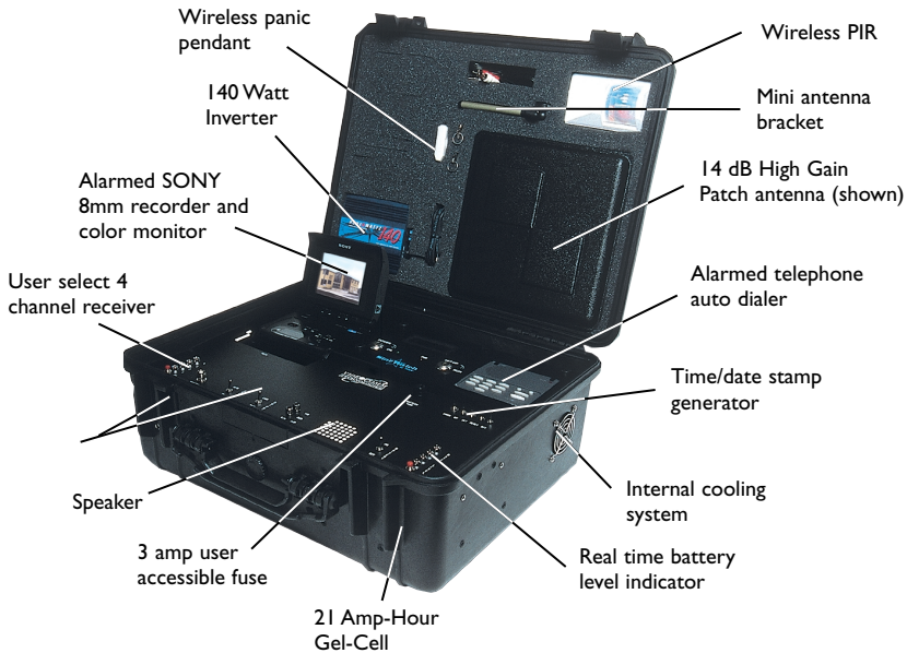
Surveillance Kit # RCV-2414sw with 14dB High Gain Antenna (shown above)
