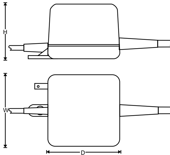
Figure 2 VC24PS-1-230 Outline Drawing
