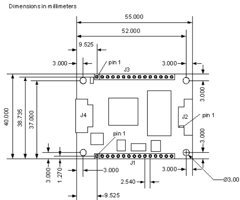
Figure 1 Main module dimensions
