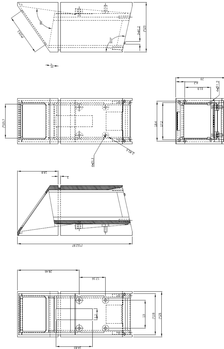
Figure 2 Sensor dimensions
