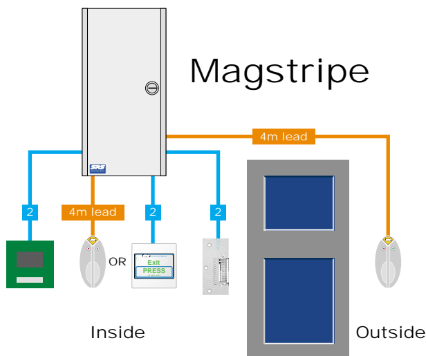
Wiring configuration of a typical door
