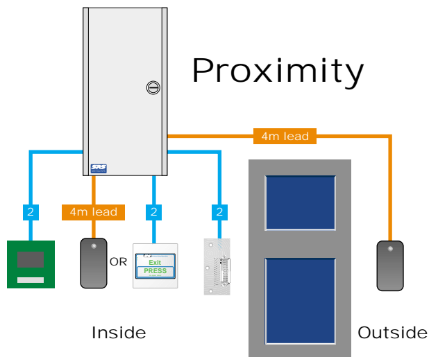
Wiring configuration of a typical door
