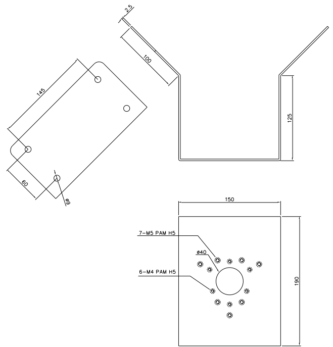
Corner Mount Adaptor
