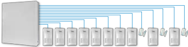
Industry Standard Busy Wiring
