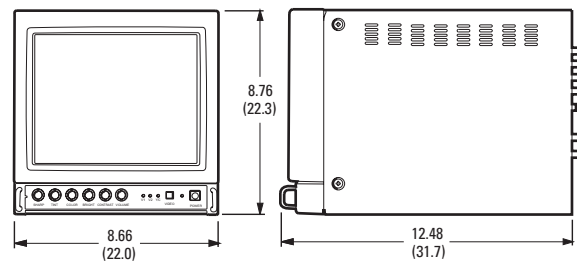
NOTE: VALUES IN PARENTHESES ARE CENTIMETERS; ALL OTHER VALUES ARE INCHES.
