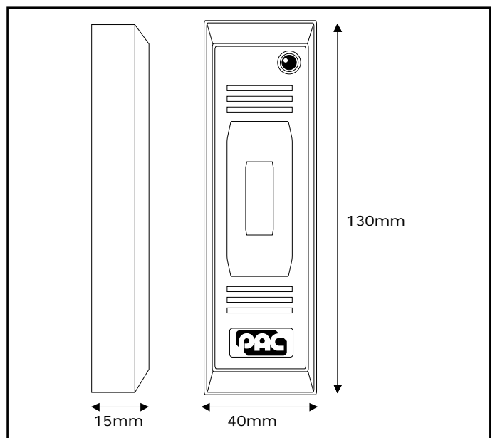
Part no. 20596 (White) 20595 (Black)
