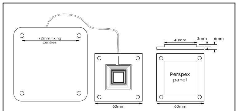
Part no. 20421
