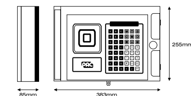
Door Controller without front panel
