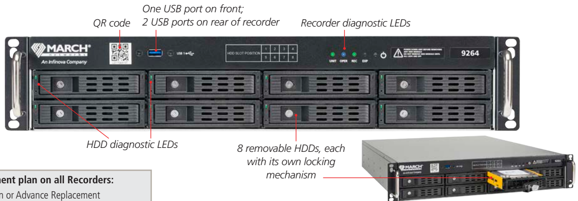
9264 Front Panel
