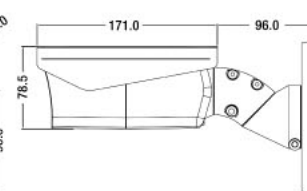
CA-PMB Pole Mount Bracket for SID-655P
