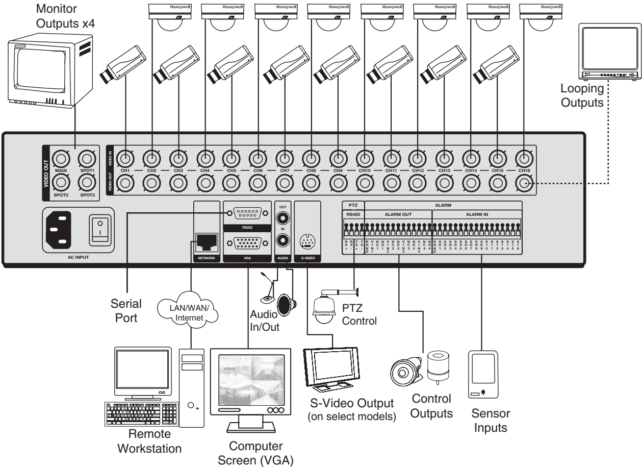
Model shown: HRDP16 16 channel DVR. Functionality will differ across the range.
