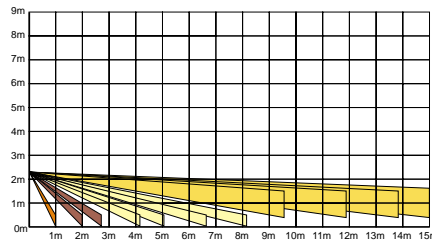
Volumetric Side elevation
