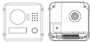
VTO2000A-C front panel and rear panel
