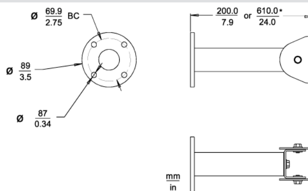
LTC 9210/01 and LTC 9223/01 Column Mount
