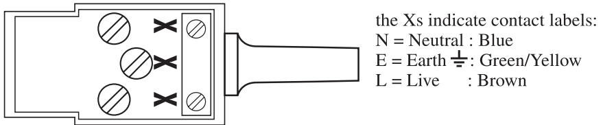
Figure 8. Internal connections on the IEC plug
