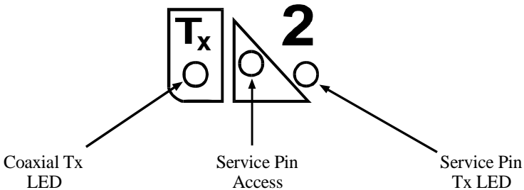
Figure 3. Channel Indicators and Service Pin Button
