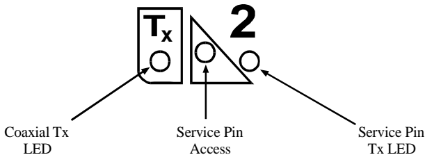
Figure A. The 2 indicator LEDs and service pin locations
