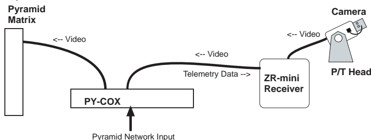
Figure 1. Illustration showing coaxial connection from matrix to receiver
