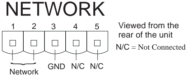
Figure 6. Network Connections
