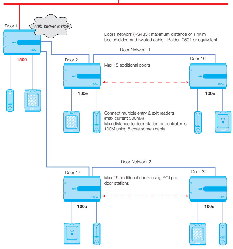
ACTpro 1500 Schematic
