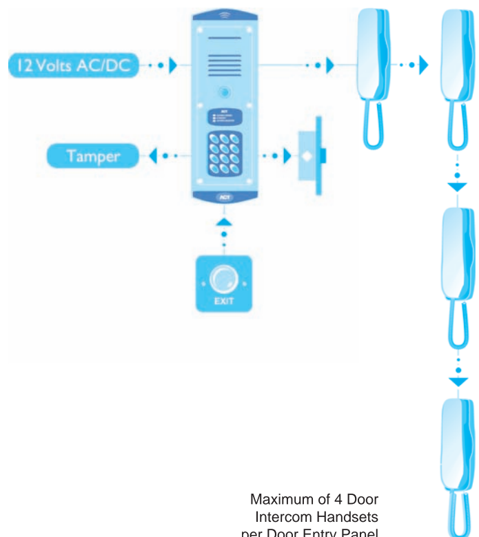
ACTentry A10 System Schematic
