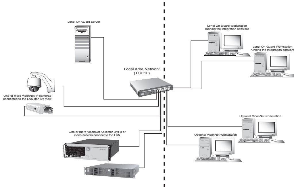
Typical Lenel OnGuard/ViconNet Network Setup
